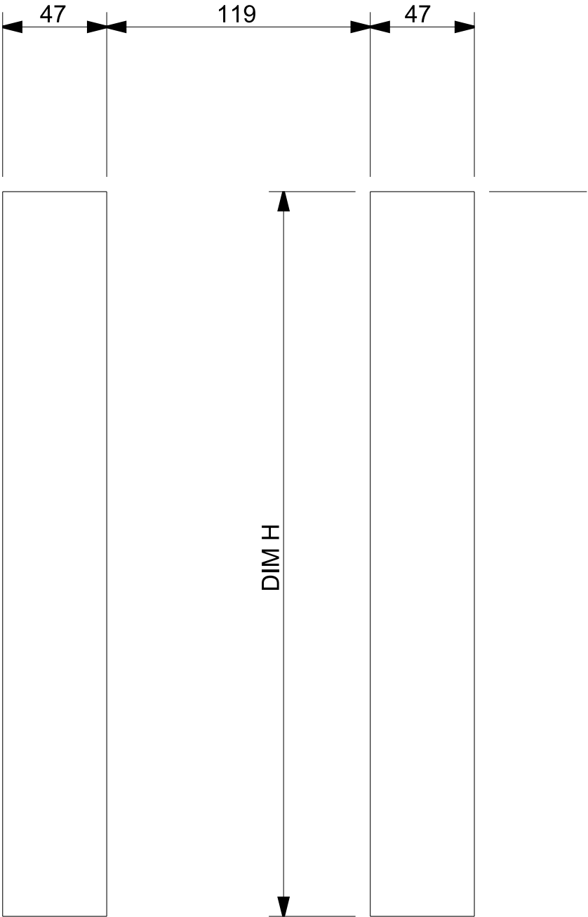
ESCUTCHEON CUTOUTS
