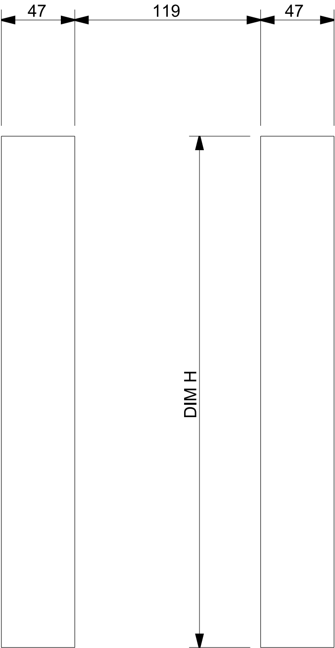
ESCUTCHEON CUTOUTS
