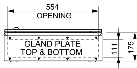
Plan view
