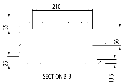
Sectional top view
