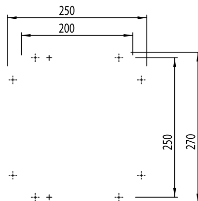
Mounting plate
