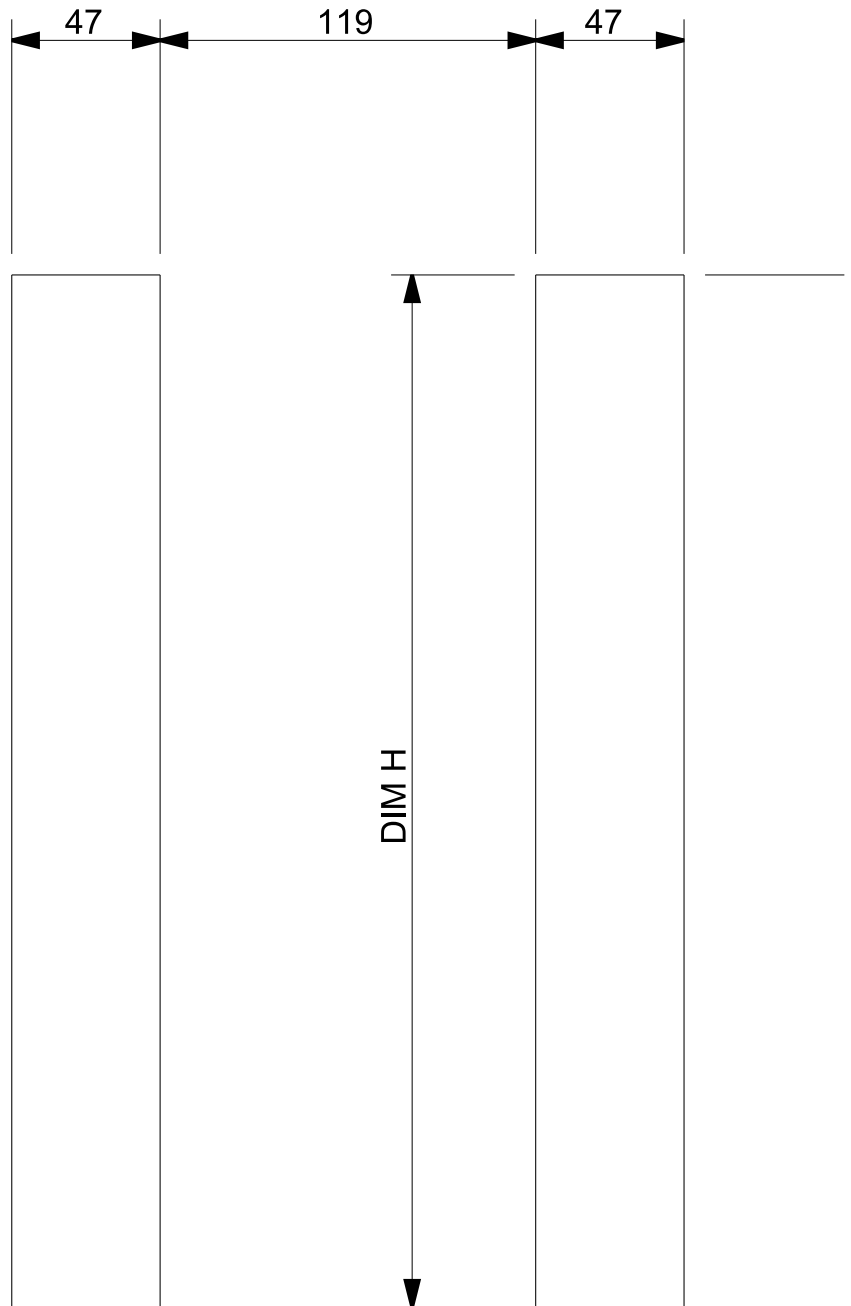
ESCUTCHEON CUTOUTS
