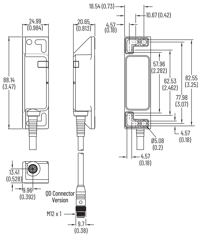
Figure 2 - Sensor Dimensions [mm (in.)]
