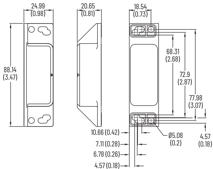
Figure 2 - Sensor Dimensions [mm (in.)]
