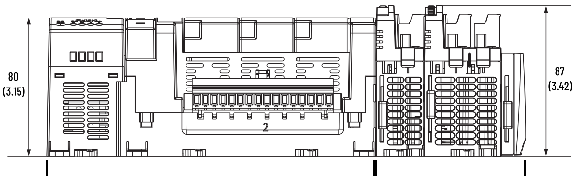
Micro830, Micro850, and Micro870 24-point Controllers (Side)
