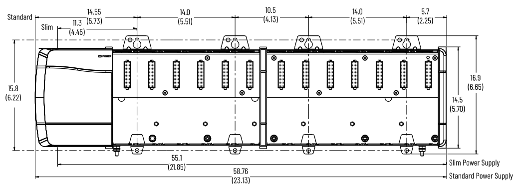
1756-A13 Chassis and Power Supply
