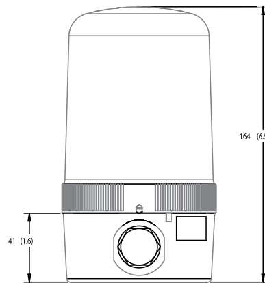
90 mm Beacon Surface Mount
