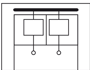
Form 3b: Terminals separated from busbars
