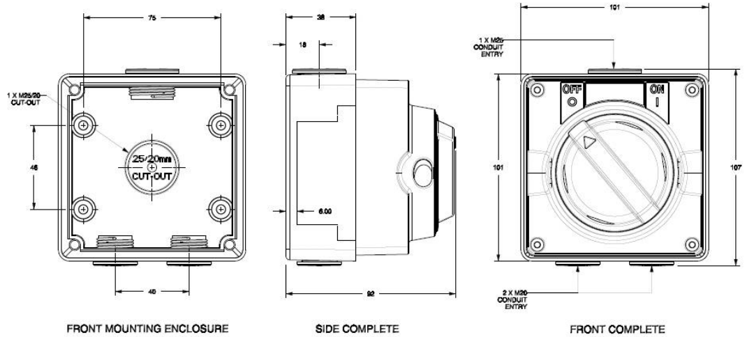
FRONT MOUNTING ENCLOSURE SIDE COMPLETE FRONT COMPLETE ISO single pole switch dimension including base
