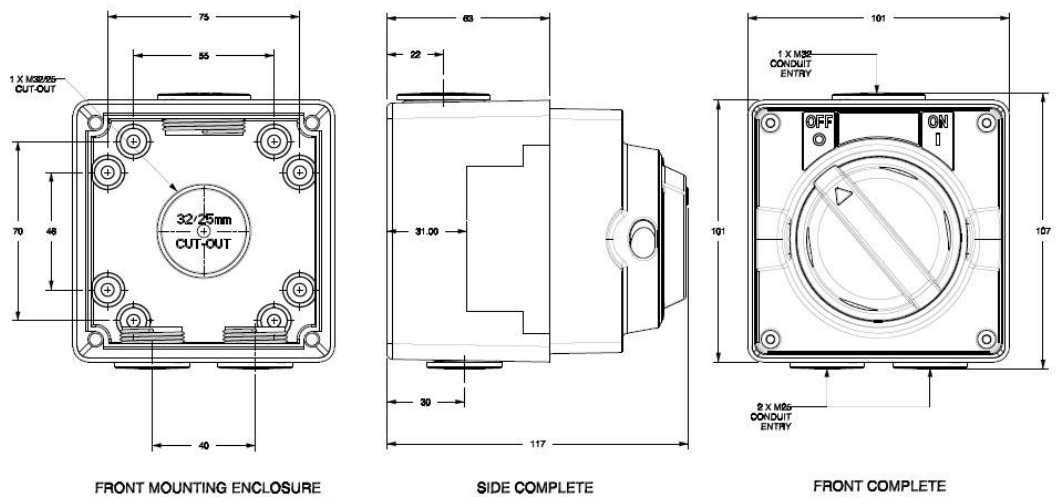
FRONT MOUNTING ENCLOSURE SIDE COMPLETE FRONT COMPLETE ISO three pole switch dimension including base
