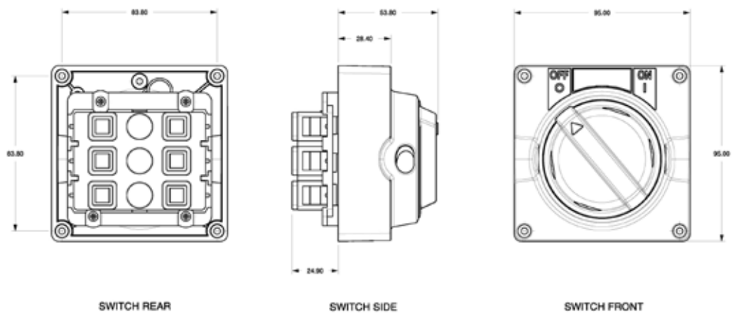
SWITCH REAR SWITCH SIDE SWITCH FRONT ISO switch dimension excluding base
