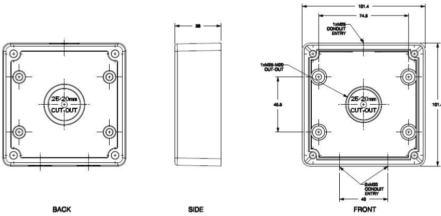
ISO single gang shallow back box dimension
