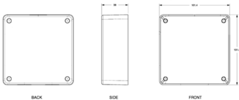
ISO single gang lid dimension
