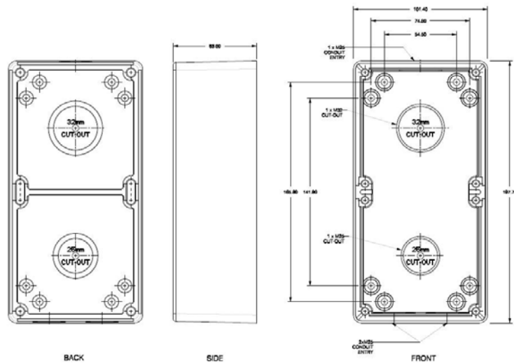
ISO two gang back box dimension
