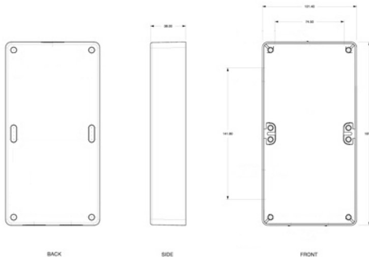
ISO two gang lid dimension
