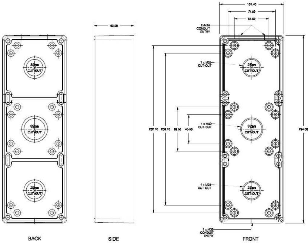
ISO three gang back box dimension
