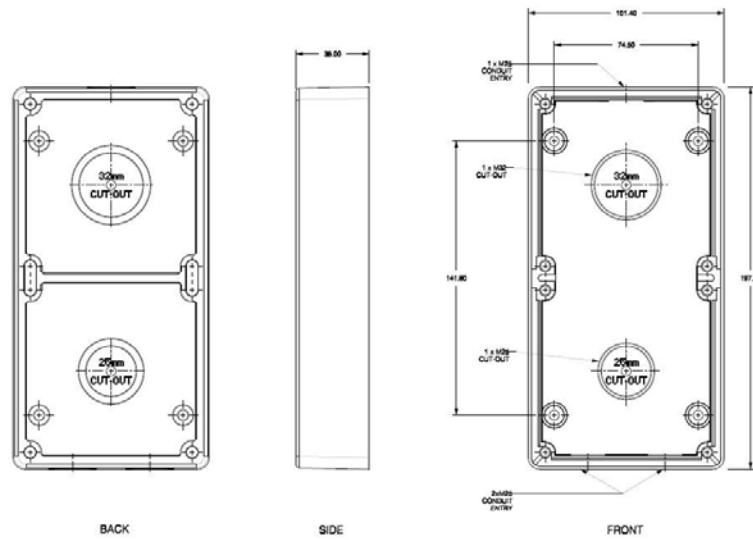
ISO two gang shallow back box dimension
